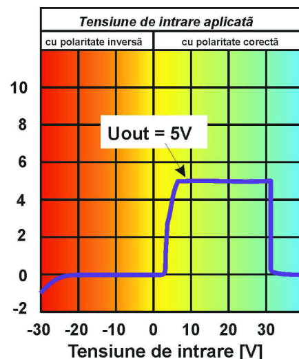
Fig. 4 Caracteristica transfer
